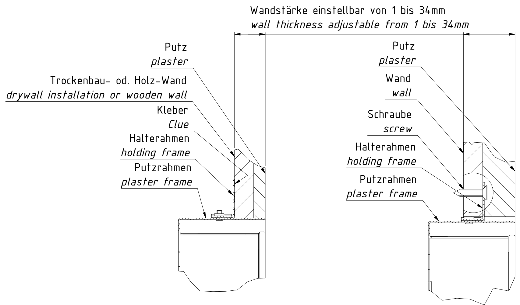
Montageart 'A' Assembly type 'A' Montageart 'B' Assembly type 'B'
