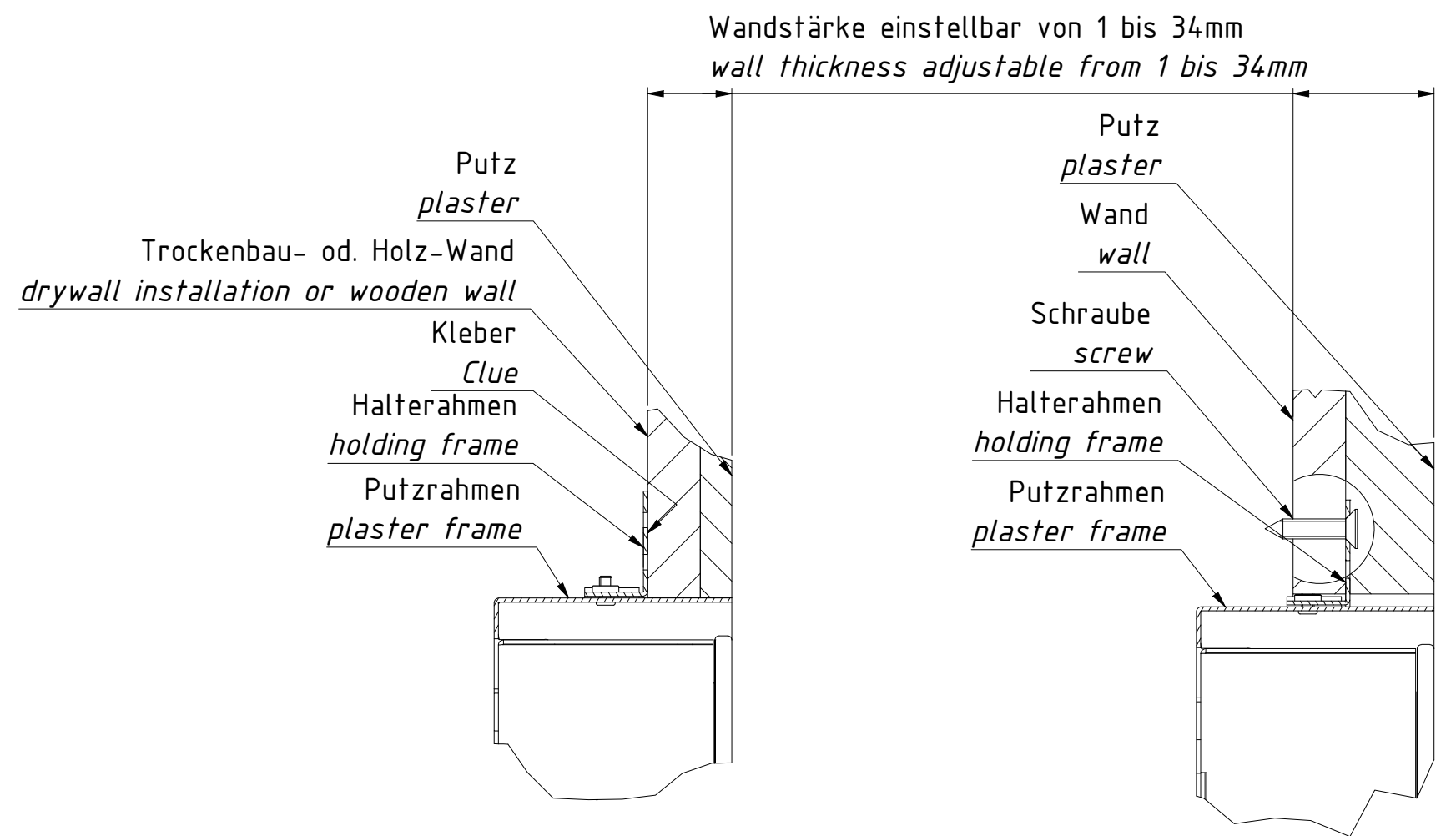
Montageart 'A' Assembly type 'A'
